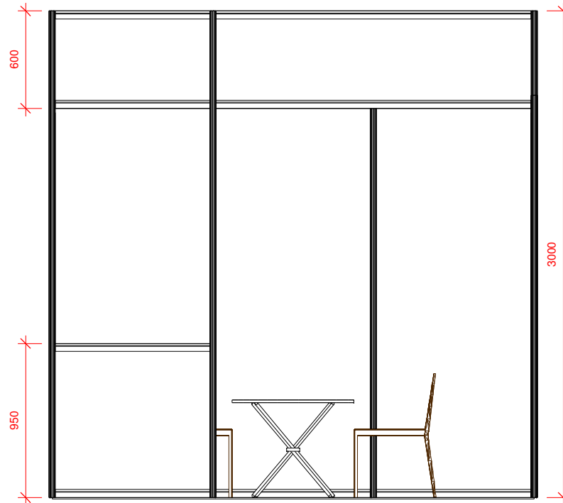
① FRONT ELEVATION 1 : 20
